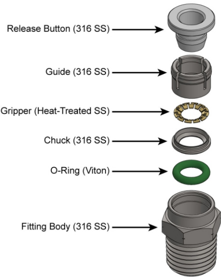
Stainless Steel (SS) Gripper-Style (W) Fitting Materials of Construction
