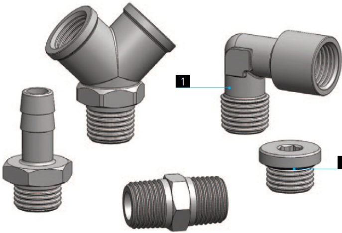
1. Fitting Body: Brass UNI EN 12164 CW614N - UNI EN 12165 CW617N Nickel Plated 2. Seals: NBR
